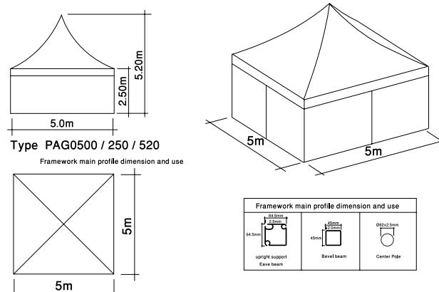
5x5m pagoda tent (Alu-PVC Structure)
